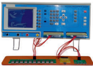
USB TESTER MODEL NO. TM-351
