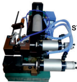
BRAIDED CABLE STRIPPING & SHEATHING MACHINE MODEL NO. TM-310, 315, 305
