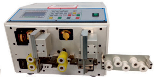
AUTOMATIC-COAXIAL / RF CABLE STRIPPER MODEL NO. TM-4806
